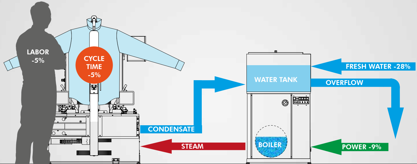
Electric boiler with condensate recovery tank
